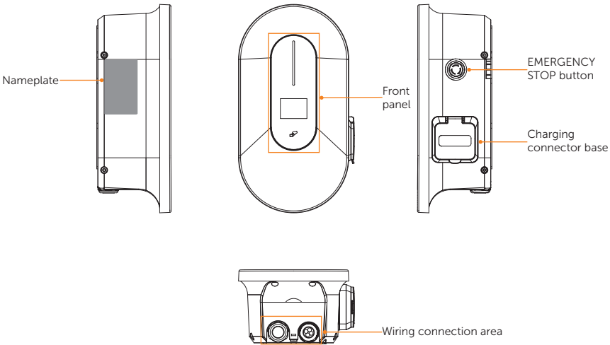
Figure 2-6 Appearance of Socket Type
