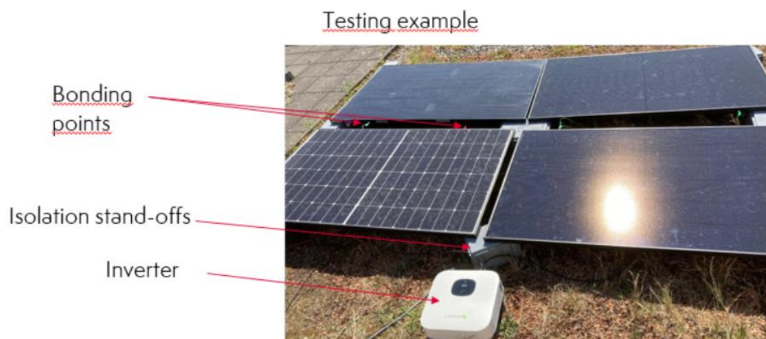
Picture 1 - Test setup example
