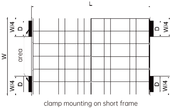
clamp mounting on short frame
