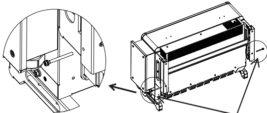
2 PCS of M6*50 bolts
